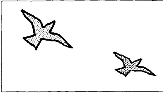
Fig. 1. Digital picture using Jordan curves.
