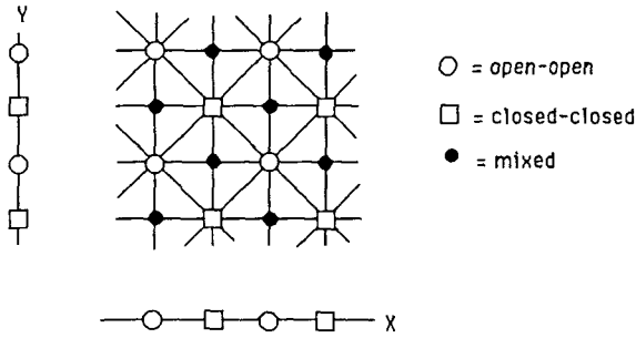
Fig. 3. A portion of a digital plane.
