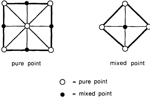
Fig. 4. The two types of adjacency sets (compare Fig. 3). Note that open–open and closed–closed points behave similarly.
